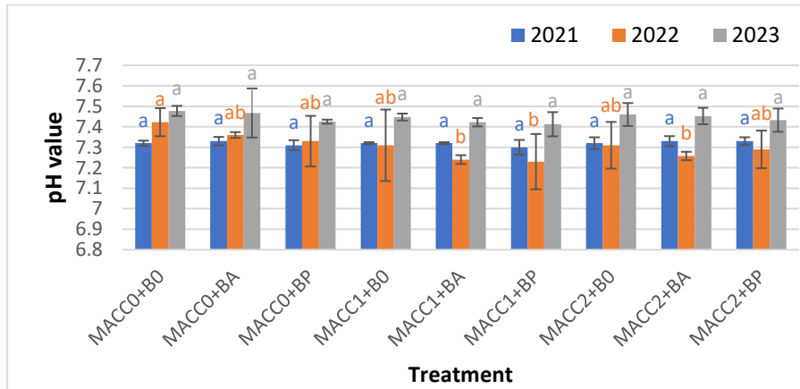
Figure 14: Effect of different application of N. linckia and PGPB on soil pH. Mean values are presented as mean \pm standard deviation. Error bars indicate standard deviation. The bars with different lowercase letters are significantly different at p \leq 0.05 by Tukey's test. Where: MACC0 and B0, control; MACC1 and MACC2, which are 0.3 g/L and 1 g/L of the N. linckia , respectively. BA and BP, which are A. lipoferum and P. florescence , respectively.
