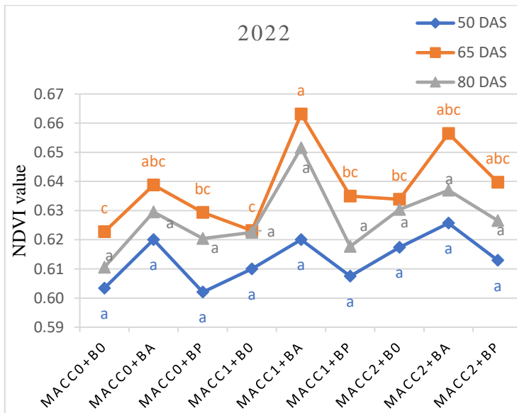
Figure 11: The NDVI value of maize ( Zea mays L.) assessed at different days after sowing (DAS) in 2022. Where: MACC0 and B0, control; MACC1 and MACC2, which are 0.3 g/L and 1 g/L of the N. linckia , respectively. BA and BP, which are A. lipoferum and P. floescence , respectively.
