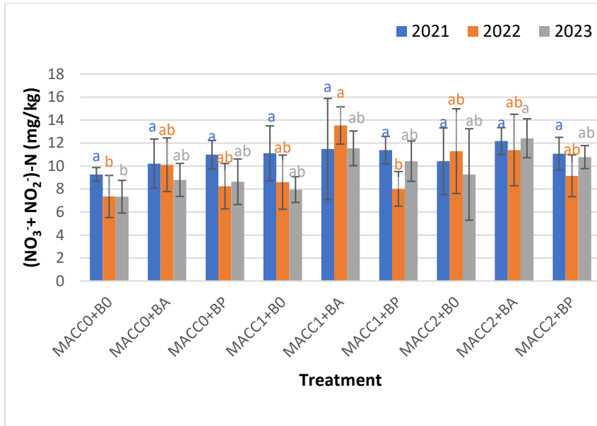
Figure 16: Effect of different application of N. linckia and PGPB on soil nitrate-nitrite-nitrogen. Mean values are presented as mean \pm standard deviation. Error bars indicate standard deviation. The bars with different lowercase letters are significantly different at p \leq 0.05 by Tukey's test. MACC0 and B0, control; MACC1 and MACC2, which are 0.3 g/L and 1 g/L of the N. linckia , respectively. BA and BP, which are A. lipoferum and P. florescence , respectively.
