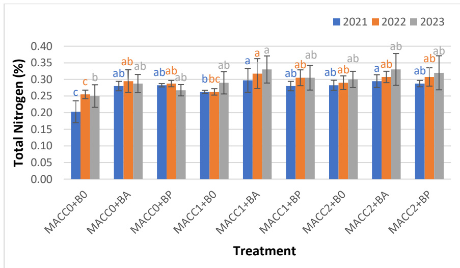
Figure 17: Effect of different application of N. linckia and PGPB on soil total nitrogen. Mean values are presented as mean \pm standard deviation. Error bars indicate standard deviation. The bars with different lowercase letters are significantly different at p \leq 0.05 by Tukey's test. Where: MACC0 and B0, control; MACC1 and MACC2, which are 0.3 g/L and 1 g/L of the N. linckia , respectively. BA and BP, which are A. lipoferum and P. florescence , respectively.
