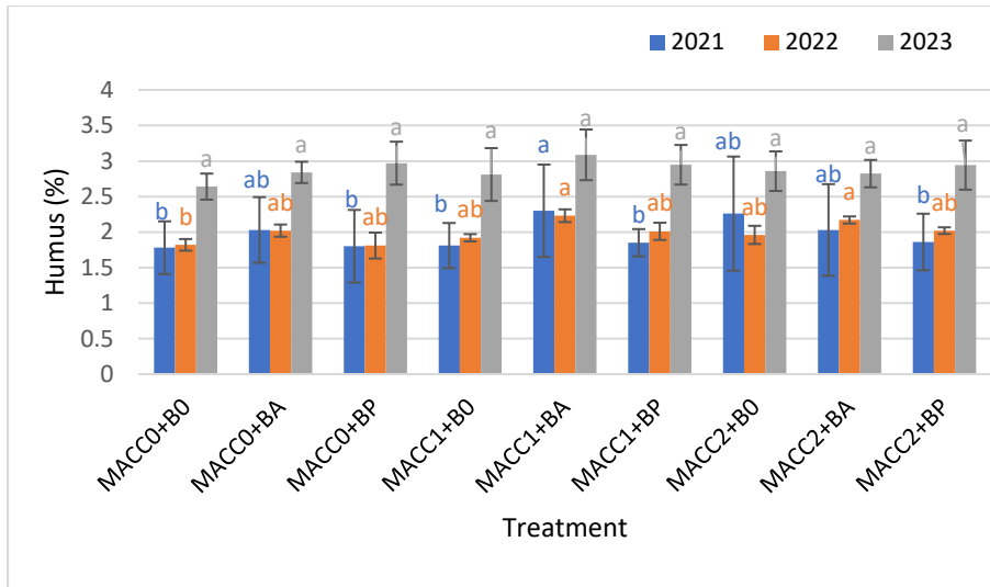
Figure 15: Effect of different application of N. linckia and PGPB on soil humus. Mean values are presented as mean \pm standard deviation. Error bars indicate standard deviation. The bars with different lowercase letters are significantly different at p \leq 0.05 by Tukey's test. MACC0 and B0, control; MACC1 and MACC2, which are 0.3 g/L and 1 g/L of the N. linckia , respectively. BA and BP, which are A. lipoferum and P. florescence , respectively.
