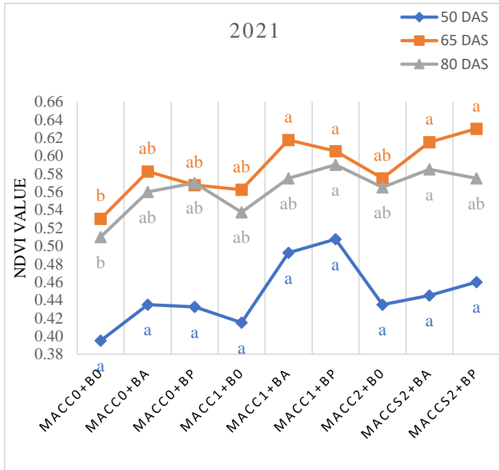
Figure 10: The NDVI value of maize ( Zea mays L.) assessed at different days after sowing (DAS) in 2021. Where: MACC0 and B0, control; MACC1 and MACC2, which are 0.3 g/L and 1 g/L of the N. linckia , respectively. BA and BP, which are A. lipoferum and P. florescence , respectively.
