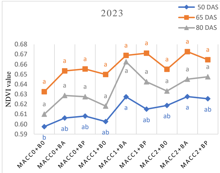
Figure 12: The NDVI value of maize ( Zea mays L.) assessed at different days after sowing (DAS) in 2023. Where: MACC0 and B0, control; MACC1 and MACC2, which are 0.3 g/L and 1 g/L of the N. linckia , respectively. BA and BP, which are A. lipoferum and P. florescence , respectively.
